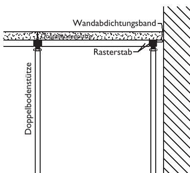
Rasterstab
