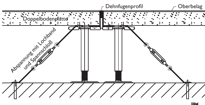
Dehnfuge
